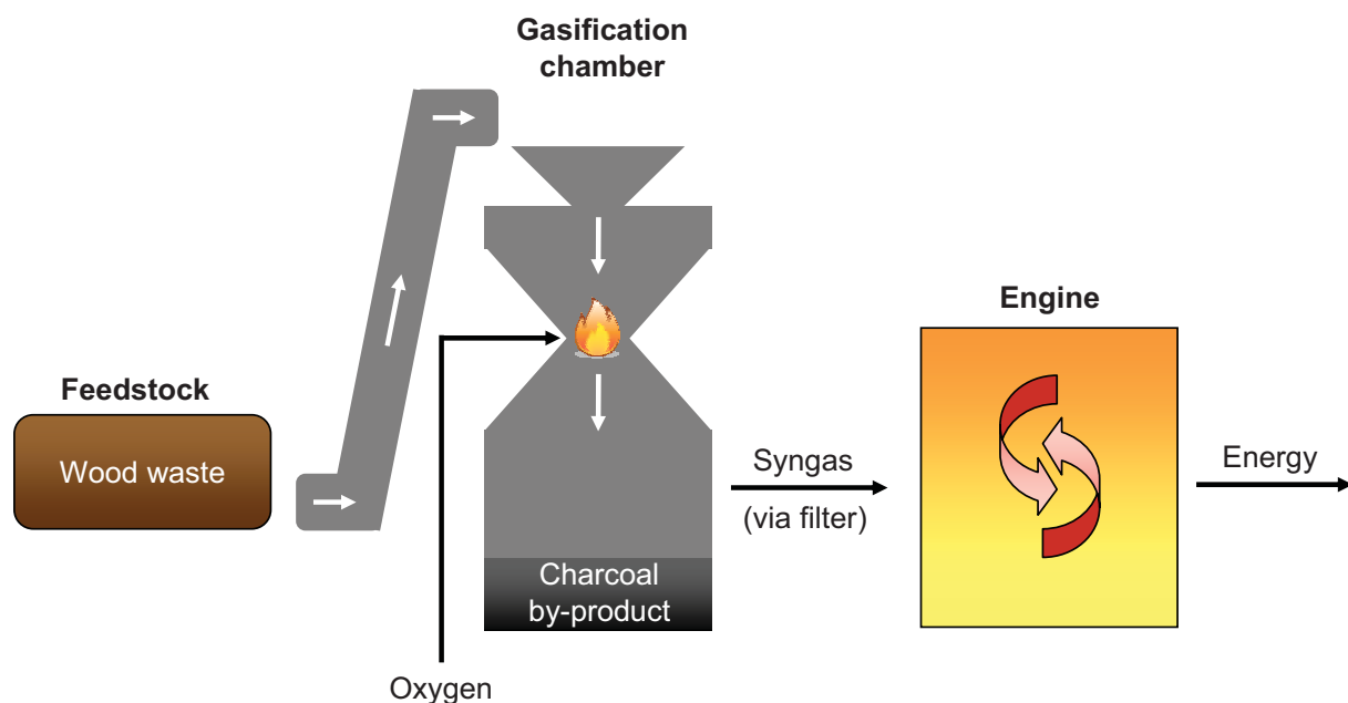
Figure 2: The gasification process
