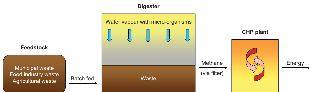
Figure 3: The anaerobic digestion process
